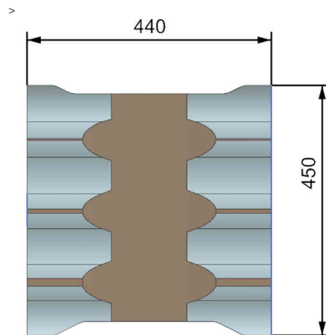
Saucer Drain Cover Mould 450mm X 440mm X 100mm
